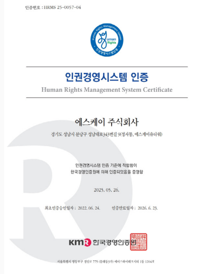
HRMS
